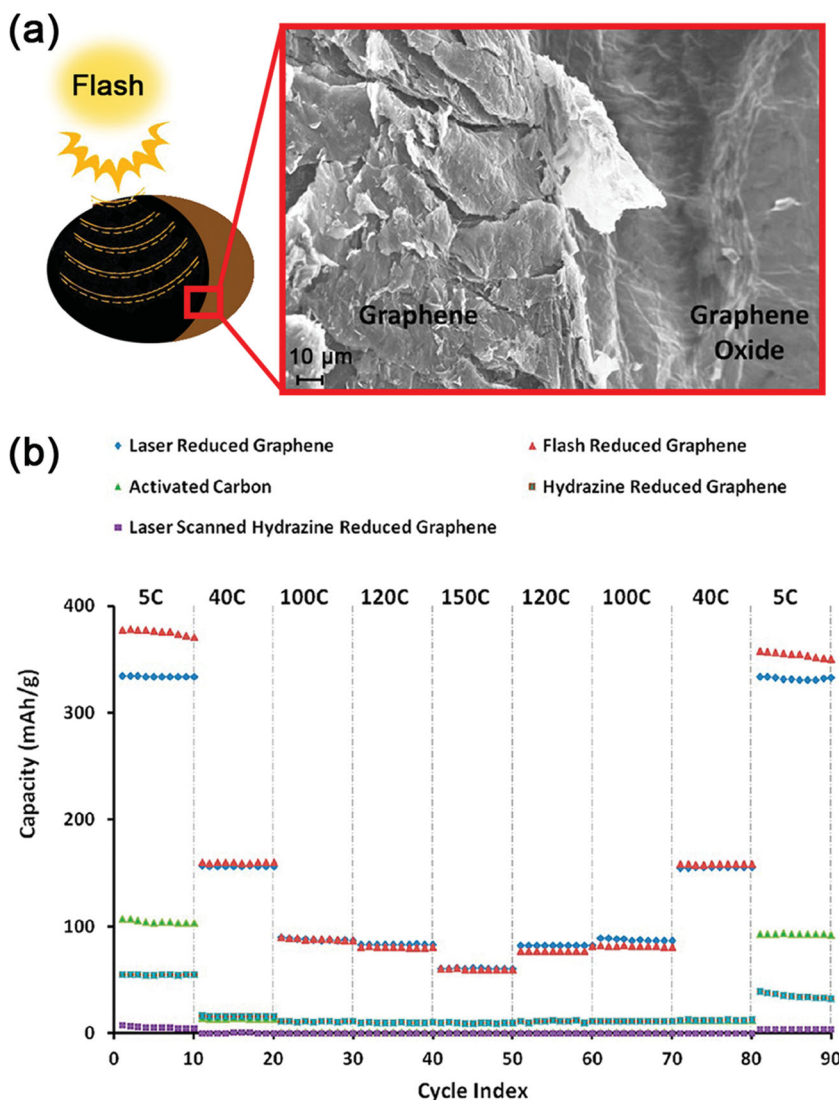
Figure 11. a) Schematic showing the flash reduction of GO and SEM image of the regions containing both flash-reduced GO and GO. b) Performance of laser- and flash-reduced graphene anodes at various C rates, compared to the performance of control samples of activated carbon, hydrazine-reduced graphene, and laser-scanned hydrazine-reduced graphene. The cells were operated for 10 cycles each at different C rates from 5 to 150 C and were then brought back to 5 C in the reverse sequence. Reproduced with permission. [166] Copyright 2012, American Chemical Society.
