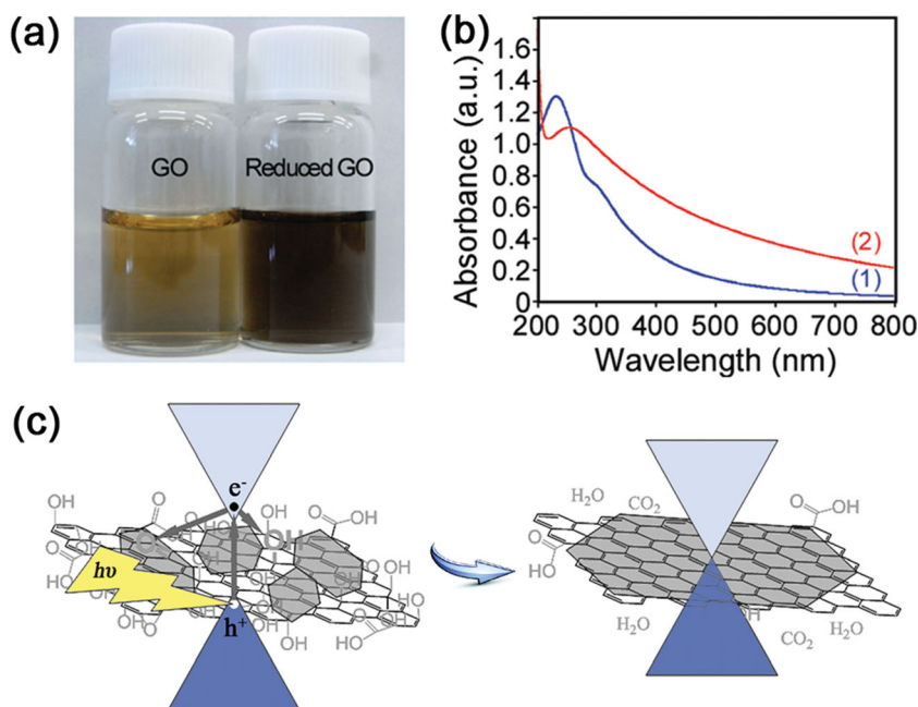
Figure 4. a) Photographs of GO and RGO solution; b) UV-vis spectra of nanosheet suspensions of (1) GO and (2) RGO prepared by photoreduction in H_2 for 2 h. Reproduced with permission. [115] Copyright 2010, American Chemical Society. c) Schematic illustration of the photochemical reduction mechanism of GO to RGO. Reproduced with permission. [84] Copyright 2012, John Wiley and Sons.
