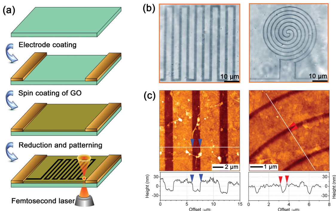
Figure 7. a) Schematic illustration of the FSLDW reduction and patterning of GO; b) optical microscopic images of different micropatterns; c) AFM image of the detail of micropatterns, the bottom two images show the profile of the micropatterns. Reproduced with permission. [87] Copyright 2010, Elsevier.
