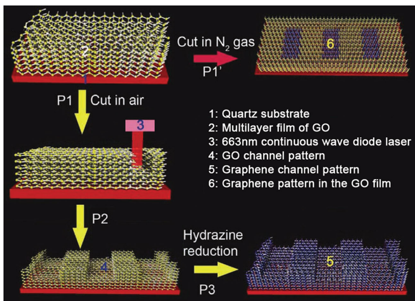
Figure 5. Schematic illustration of the cutting and patterning of GO nanosheets by a focused laser beam. For simplicity of the illustration, the hydroxyl, ether, and carboxylic groups of GO were omitted, and yellow represents GO and blue represents graphene. Reproduced with permission. [122] Copyright 2010, John Wiley and Sons.
