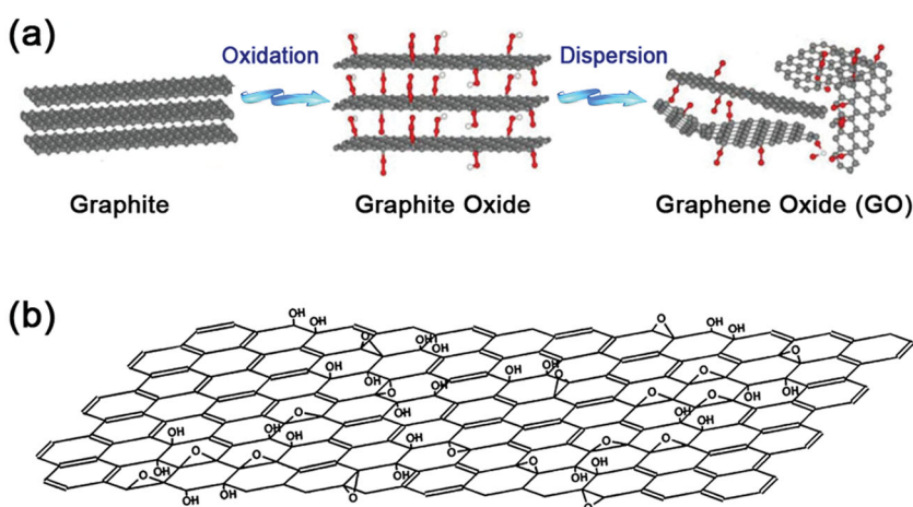
Figure 1. a) Schematic illustration of the preparation of GO from graphite; b) Schematic illustration of the structural model of a GO sheet. Reproduced with permission. [91] Copyright 1998, Elsevier.
