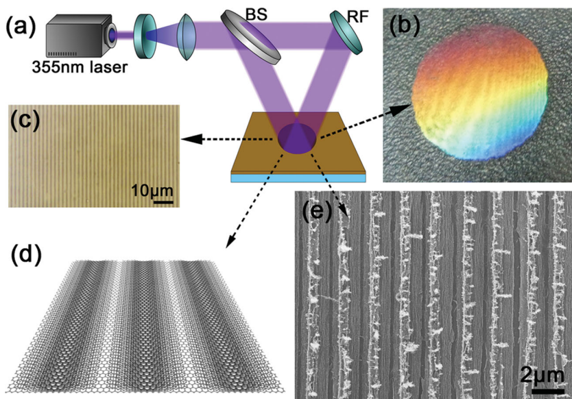
Figure 9. a) A schematic illustration of the two-beam laser interference system for the fabrication of superhydrophobic graphene films. b) A photograph of an as-patterned graphene film. The structural color can be observed by the naked eye. c) An optical microscopic image of the graphene pattern. d) A schematic illustration of the graphene surface after two-beam laser interference treatment. e) An SEM image of the superhydrophobic and iridescent graphene film. Reproduced with permission. [151] Copyright 2012, John Wiley and Sons.
