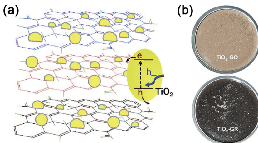
Figure 3. a) Schematic illustration of TiO 2 -assisted photoreduction of GO under UV excitation; b) photographs of TiO 2 -GO composite before and after reduction. Reproduced with permission. [69] Copyright 2008, American Chemical Society.
