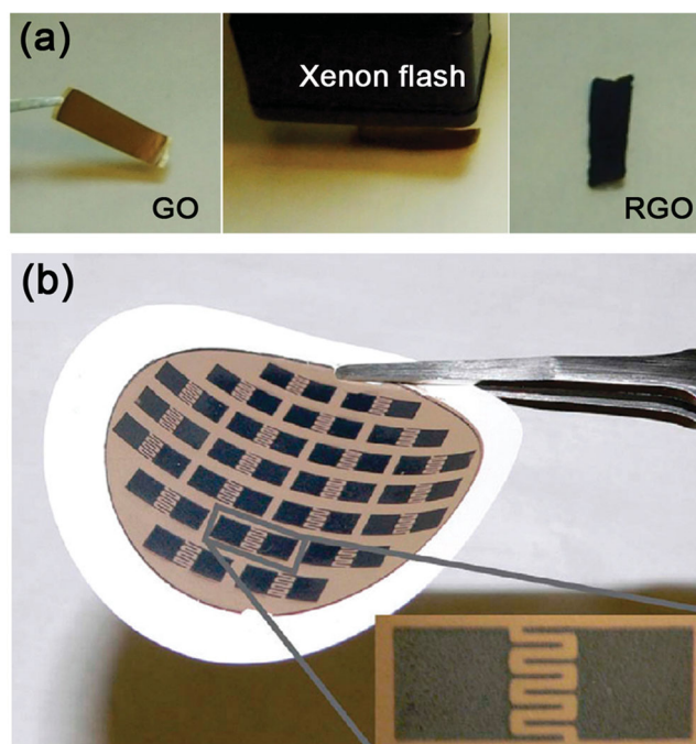
Figure 2. Flash reduction of GO. a) Photographs of GO, flash reduction of GO and RGO, from left to right; b) photograph of the arrays of RGO/polystyrene interdigitated electrodes fabricated on a 1.5 inch diameter GO/polystyrene thin film deposited on a Nylon filter paper. The inset shows the close up view of one set of such electrode. Reproduced with permission. [81] Copyright 2008, American Chemical Society.
