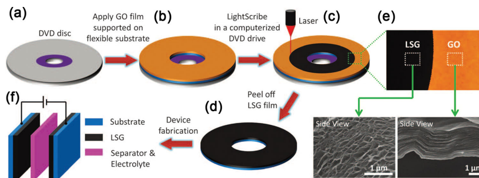
Figure 6. Schematic illustration of the fabrication of laser-scribed RGO electrochemical capacitors. a–d) A GO film supported on a flexible substrate is placed on top of a LightScribe-enabled DVD media disc, and a computer image is then laser-irradiated on the GO film in a computerized LightScribe DVD drive. e) The GO film changes from golden brown to black as it is reduced to RGO. The low-power infrared laser changes the stacked GO sheets immediately into well-exfoliated few-layered laser scribed graphene film, as shown in the cross-sectional SEM images. f) A symmetric EC is constructed from two identical LSG electrodes, ion-porous separator, and electrolyte. Reproduced with permission. [127] Copyright 2012, American Association for the Advancement of Science.
